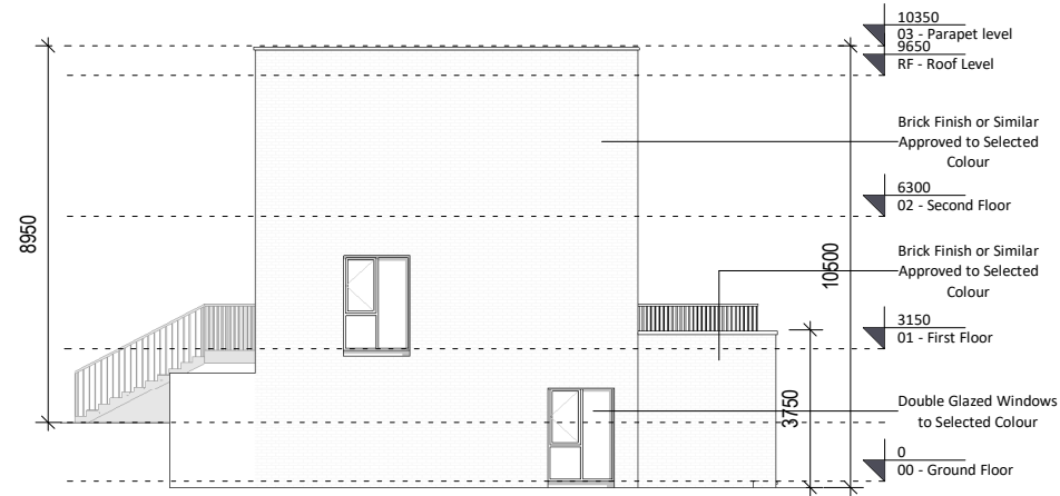
② Left Elevation 1 : 200
