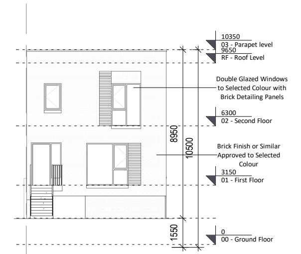
③ Rear Elevation 1 : 200
